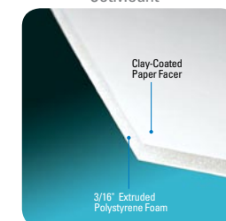
Foam-X Recovery
